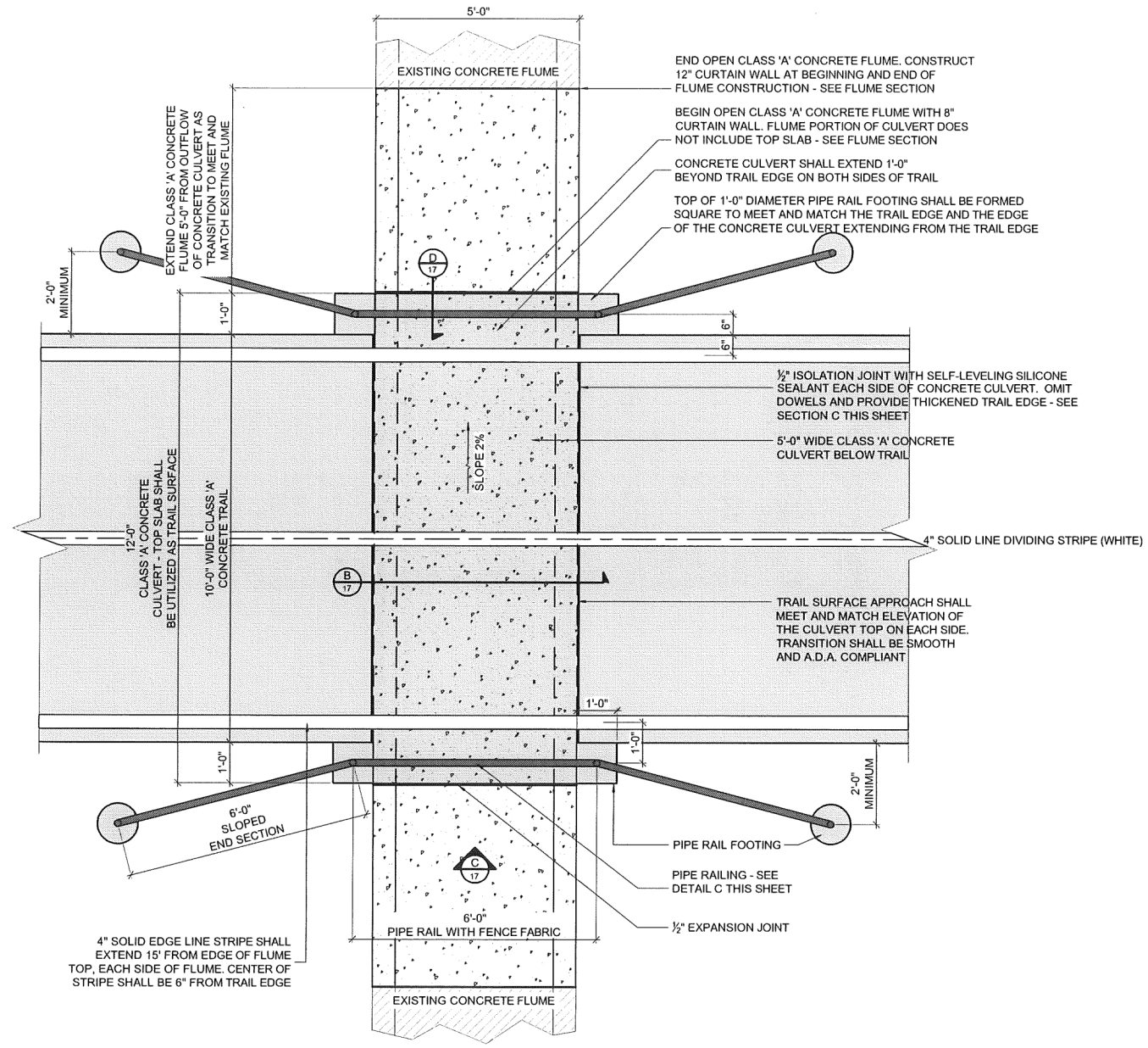
A PLAN - CONCRETE FLUME CROSSING 17 NOT TO SCALE
