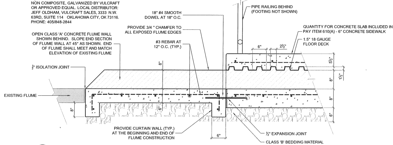
B SECTION - CONCRETE FLUME CROSSING 17 NOT TO SCALE
