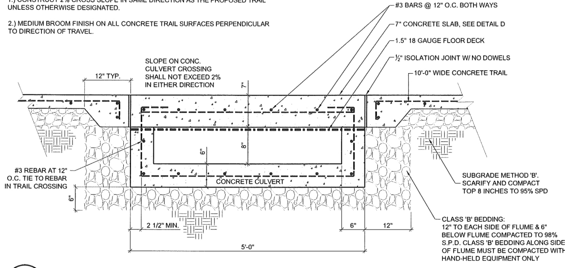
C DETAIL - STANDARD METAL PIPE RAILING AT CONCRETE FLUME CROSSING 17 NOT TO SCALE
